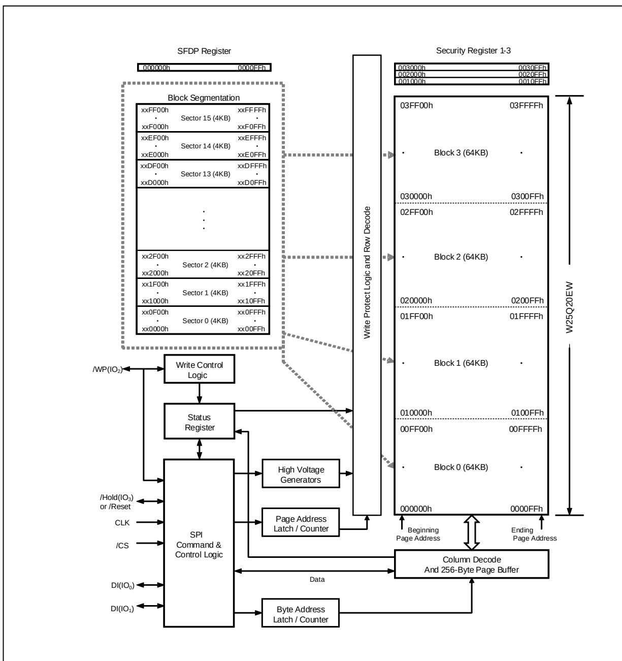
Figure 2.W25Q20EW Serial Flash Memory Block Diagram
